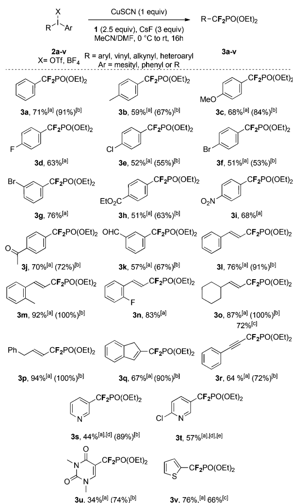
Scheme 2. Scope of the reaction (0.25–0.5 mmol scale). [a] Yield of isolated products. [b] NMR yields determined by using \alpha,\alpha,\alpha -trifluorotoluene as internal standard. [c] Reactions performed on 3.4 mmol scale. [d] 1,10-phenanthroline (1 equiv) was added. [e] Contaminated with 10% of an unknown product.
